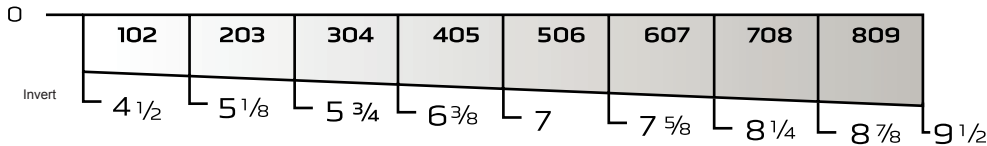
TYPICAL MODULAR LAYOUT OF A 7000 SERIES SLOT DRAIN® SYSTEM (Sections fit together as illustrated below)
