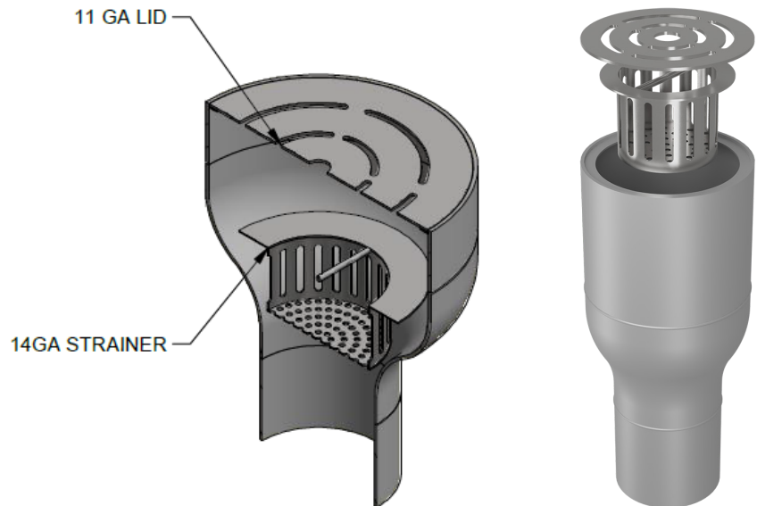
TYPICAL PROFILE OF A FOODSAFE HUB DRAIN
